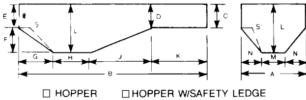
HOPPER HOPPER W/SAFETY LEDGE
